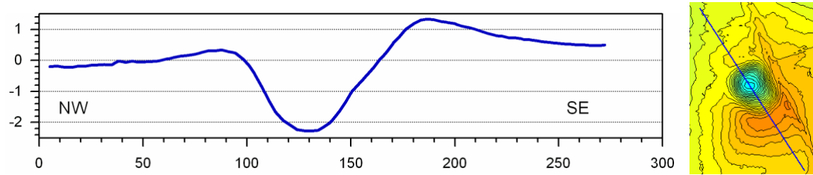
Fig. 24. Residual topography and diametral profile. The asymmetry may be explained by a doublet broken impactor or a strongly oblique impact, which has a companion feature on the Moon (Figs. 26).
