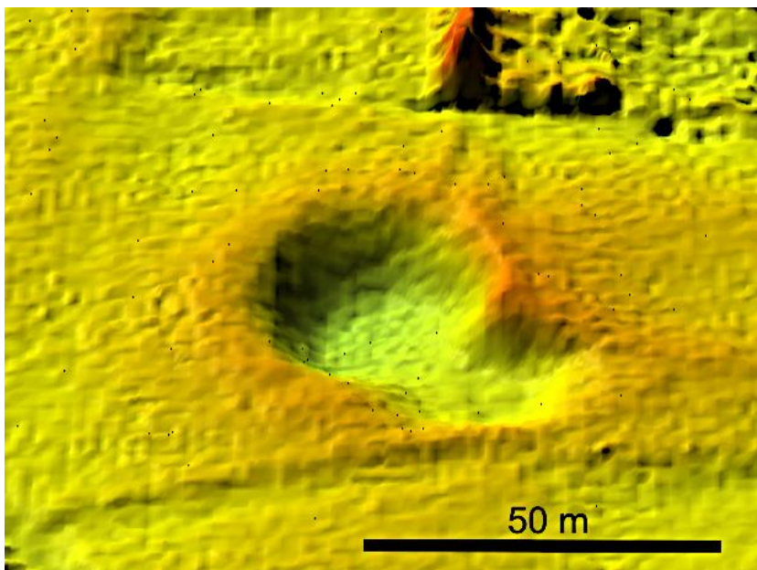
Palling SW doublet crater
