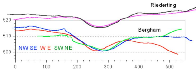
Fig. 14. There is a striking similarity between the Riederting crater (Fig. 7) and the Bergham crater (Fig. to the right), The same length and height scale applies to both structures.
