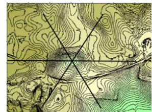
Fig. 14. There is a striking similarity between the Riederting crater (Fig. 7) and the Bergham crater (Fig. to the right), The same length and height scale applies to both structures.
