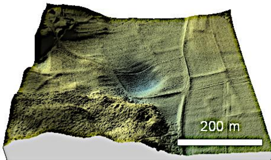
Fig. 4. Digital Terrain Model DGM 1 of the Riederting impact crater; topographic map.
