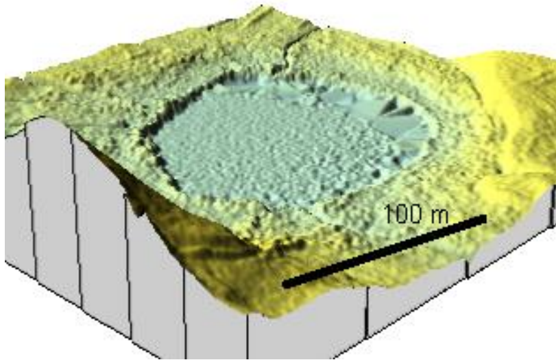
Lake Laubensee crater
