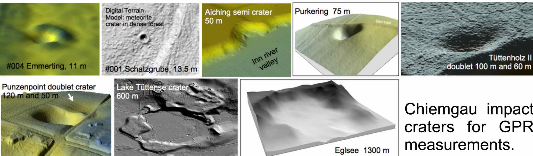
Surface 3D images are from the Digital Terrain Model DGM 1. Note the strong exaggeration. Meter specifications are rim wall diameters. The Emmerting, Aiching, Punzenpoint, Lake Tüttensee and Eglsee craters are discussed here on the poster.
