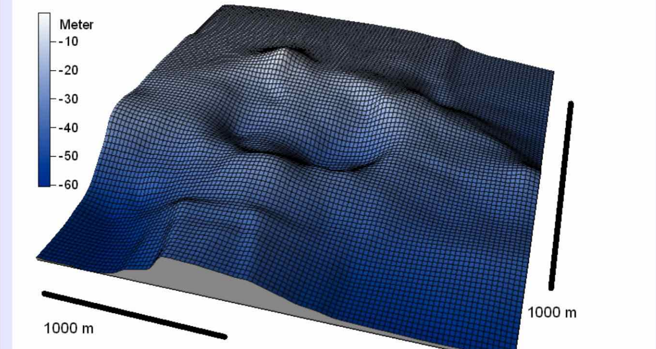
The doublet meteorite impact crater at the bottom of Lake Chiemsee. From echo sounder measurements.
